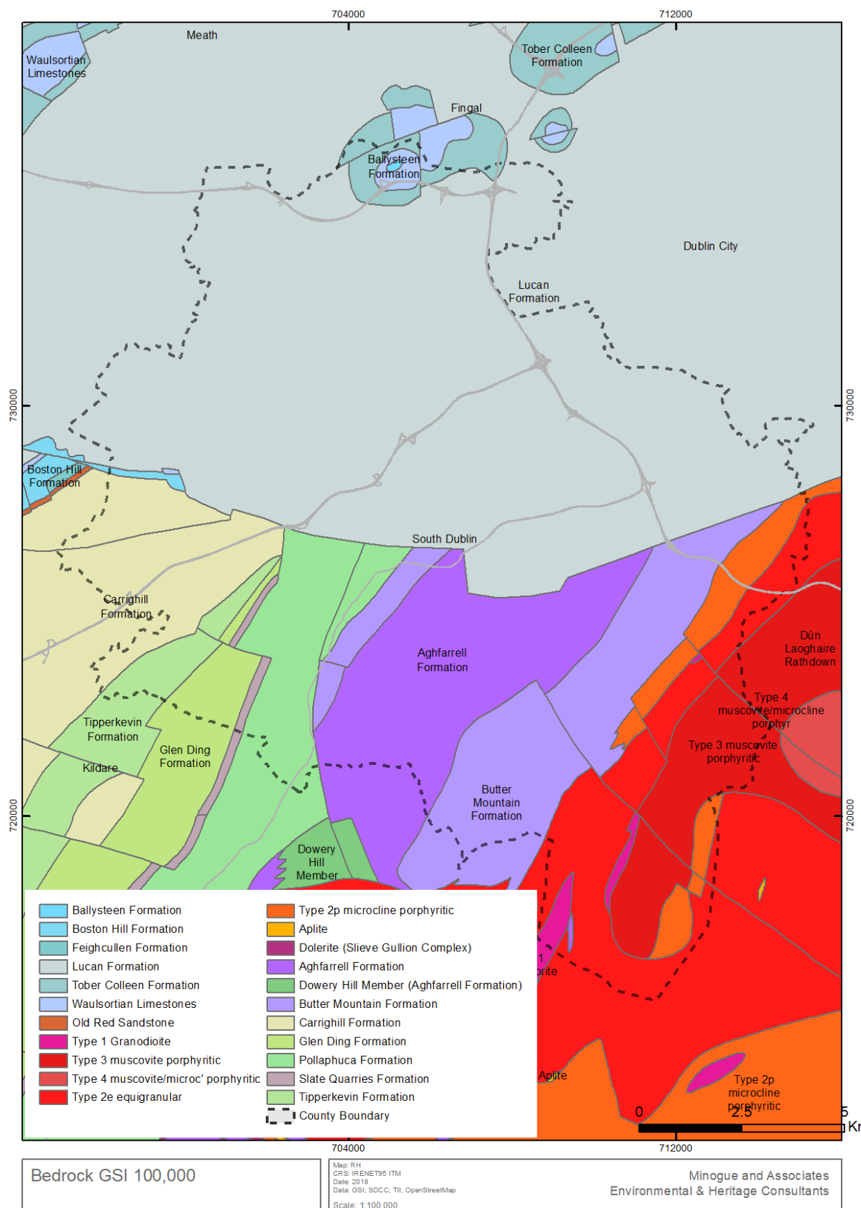
FIGURE 12 BEDROCK GEOLOGY
